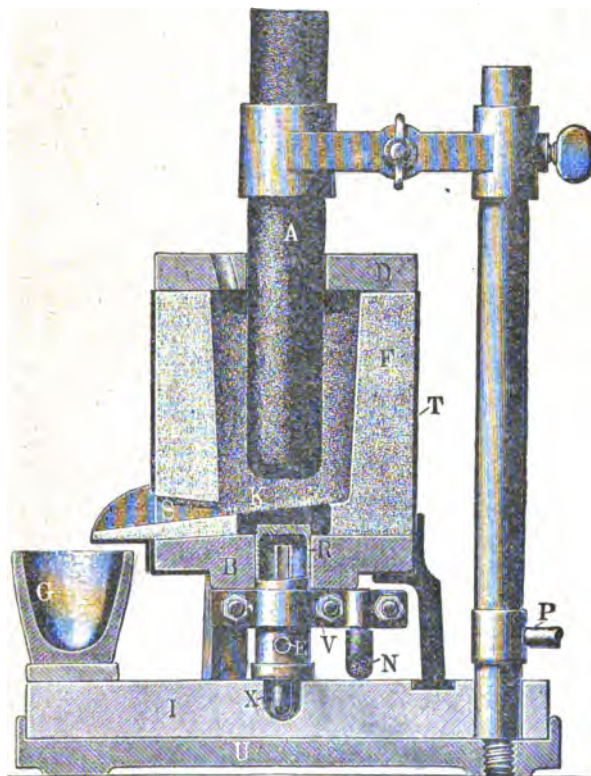
Fig. 154. — Four Borchers.
